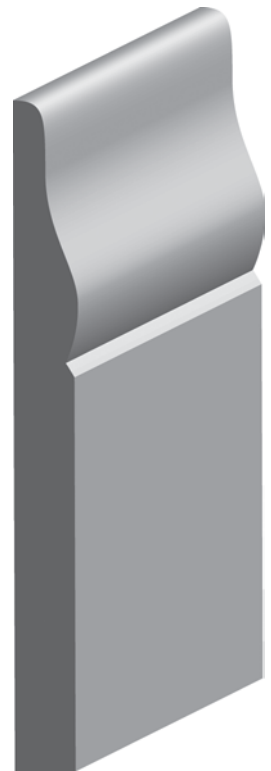
311M 7/16" x 3 1/2" MDF #711 Base
